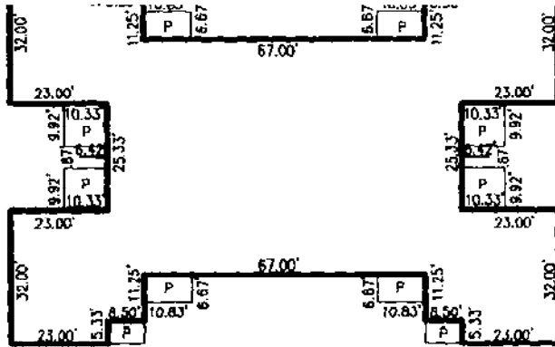
TYPICAL BUILDING DETAIL SCALE 1"=30'
